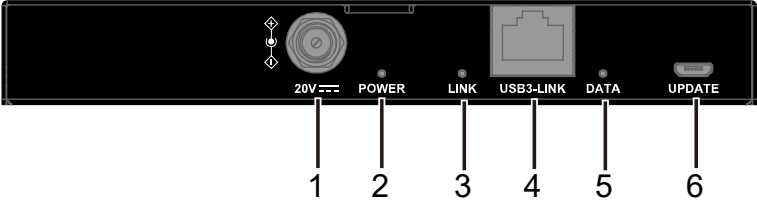
Rear Panel
